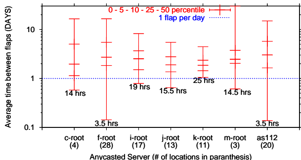
Figure 5: Percentiles for the average time between flaps for all the anycasted destinations
